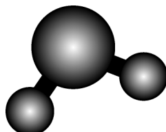
Fig.1. Schematic diagram of H 2 O molecule
